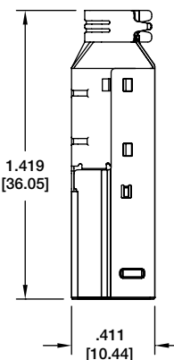
USB 3.0, TYPE B PLUG
